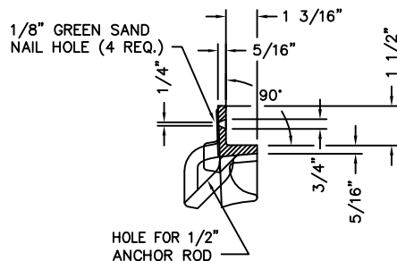
TYPICAL FRAME SECTION (SCALE: 1/4"=1")
