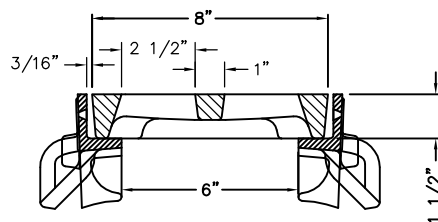
R-4990-AX TYPICAL SECTION TYPE "P" GRATE w/ TYPE "B" FRAME (SCALE: 1/4"=1")
